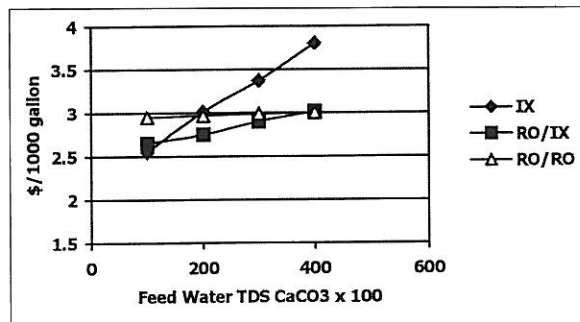
Figure 6. Comparison of RO/IX, and RO/RO for Different TDS Waters
