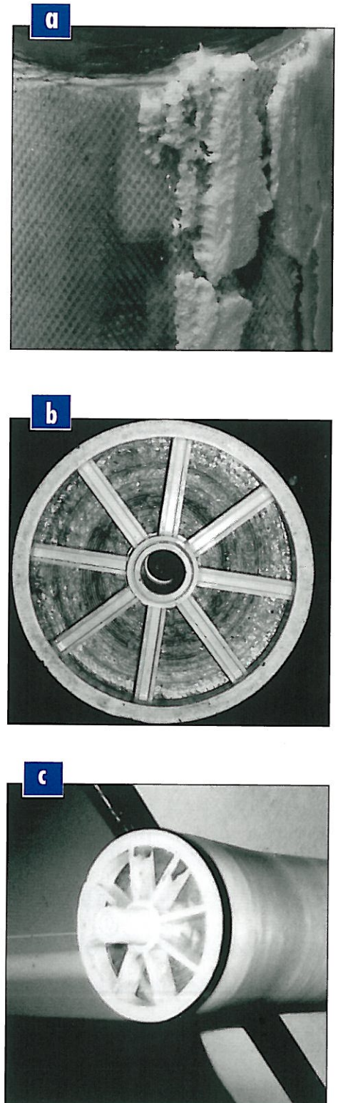
Figure 3. Fouled Membranes: a) Mineral Scale, b) Bacteria, and c) Iron
