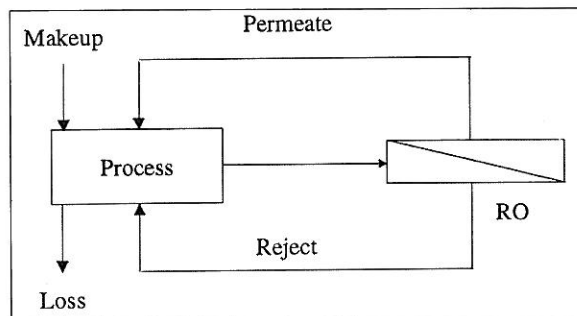
Figure 7. Total Recycle of Reject and Permeate Streams
