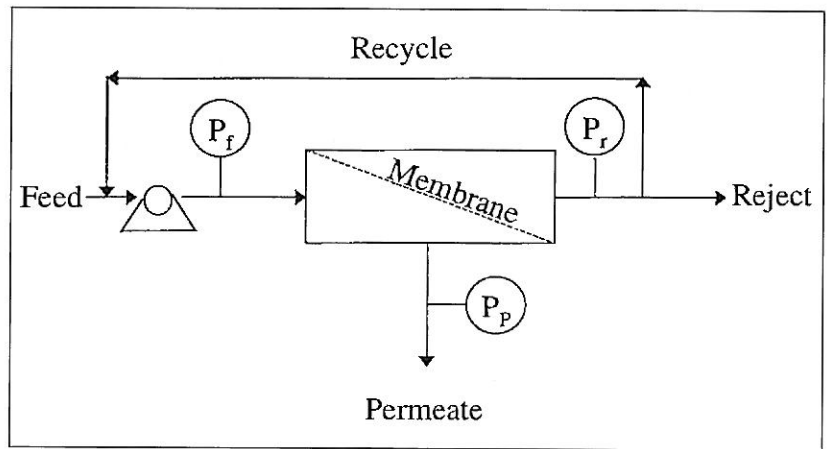
Figure 1. Fluid Streams in RO Operation
