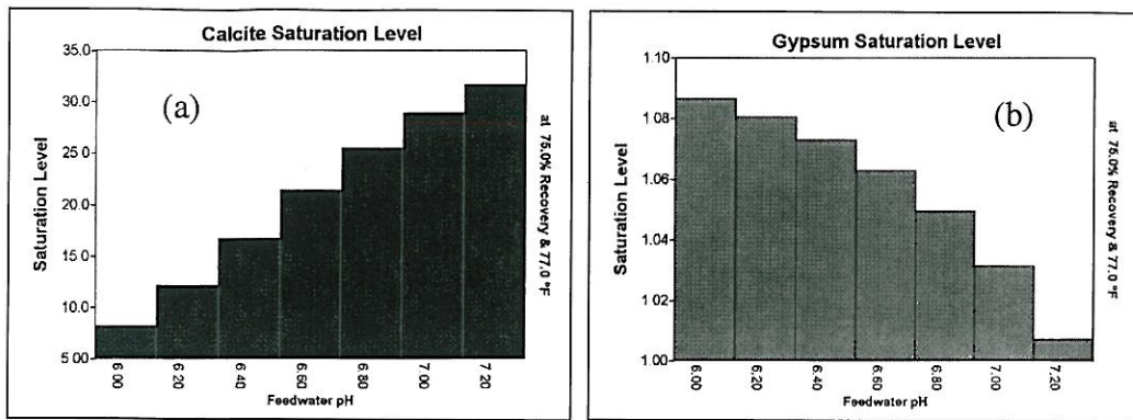
Figure 4. Effect of pH on Calcite (a) and Gypsum (B) Saturation Levels
