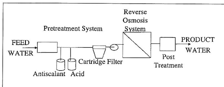
Figure 2. Fluid Streams in RO Operation
